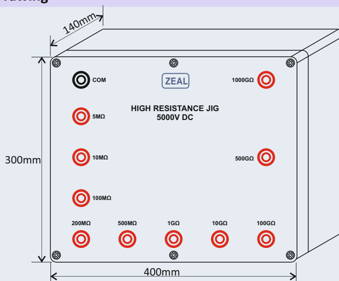
Fig. Isometric View
